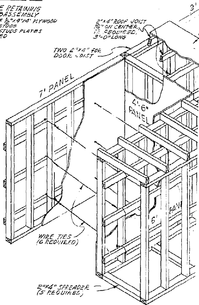
END WALL & ENTRANCE
